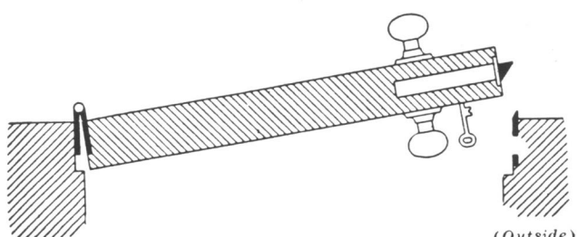
(Fig. 3) Left hand door, left hand lock
