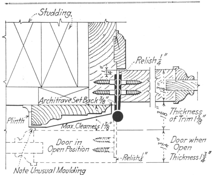
Fig. 85—Detail drawing showing how to determine proper size butt for a door
