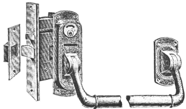
Fig. 74—Fire exit bolt for doors used for entrance and exit opening out. Door pull on outside
