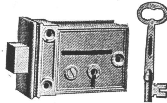
(Fig. 11) Example of the dead lock type
