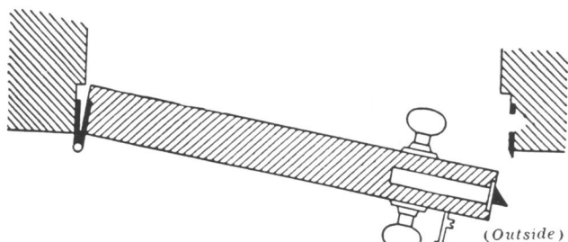
(Fig. 4) Left hand door (reverse), left hand reverse bevel lock
