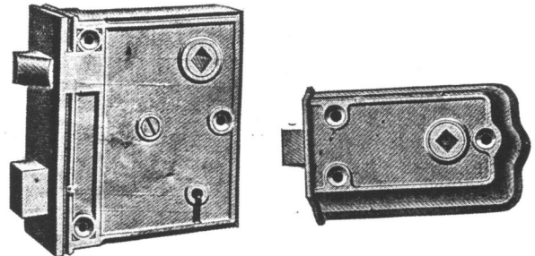
At left (Fig. 2), Janus-faced rim lock. At right (Fig. 3), single-faced rim lock
