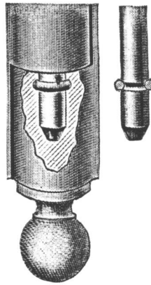
At left—Fig. 86 — Non - rising pin. At right— Fig. 87—Self re- taining pin
