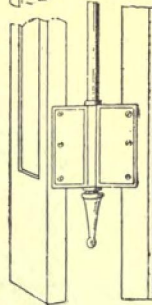
Fig. 110b. Single-acting Torsion Spring-Butt.
