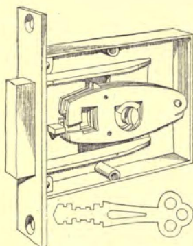
Fig. 299. Standard Store-door Lock. Yale & Towne Mfg. Co.
