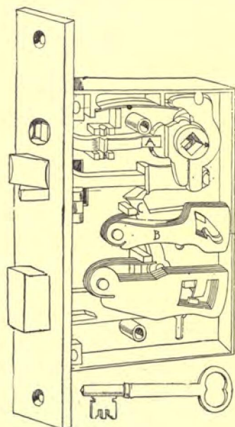
Fig. 317. Front-Door Lock. P. & F. Corbin.
