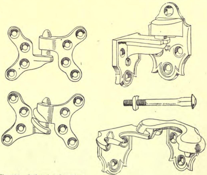
Fig. 439. Self-closing Gate-hinge, St. Louis Pattern. Shepard Hardware Co.
