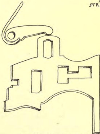
Fig. 285. Compound Lever.
