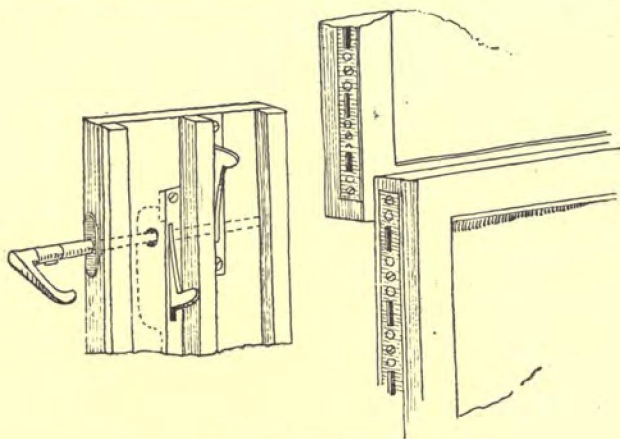
Fig. 211. Atwell Sash-fast.
