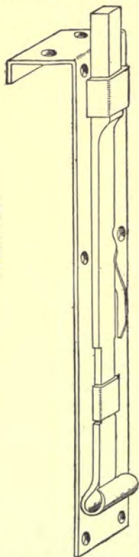
Fig. 31. Square Bolt, with Spring.
