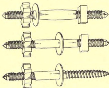
Fig. 19. Joint-bolts.
