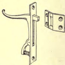
Fig. 444. Mortise Gate-latch. Ireland Mfg. Co.
