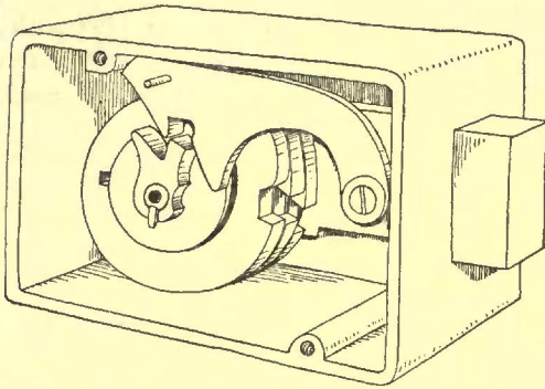
Fig. 343. Dial-Lock. Damon Safe and Lock Works.
