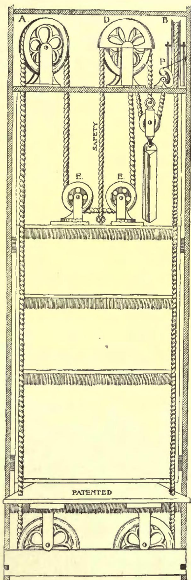
Fig. 454. New York Safety Dumb-waiter. Edw. E. R. Butts Storm Spring Co. Arch Library
