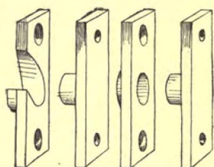
Fig. 263. Sash-centres or Transom-hinges.
